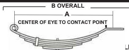
2 1/2" WIDE HAS ONE LEAF ON END
