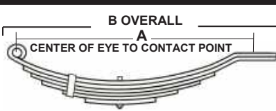
2" WIDE HAS TWO LEAFS ON END FLAT END
